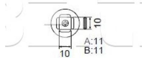
A1188B PLCC 9 x 9 (20 Pins)
