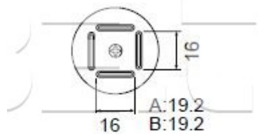
A1181B BQFP 19 x 19
