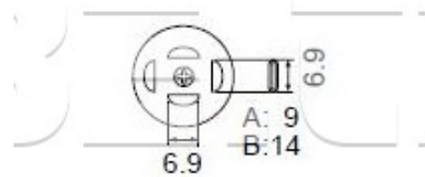
A1139B PLCC 12.5 x 7.3 (18 Pins)
